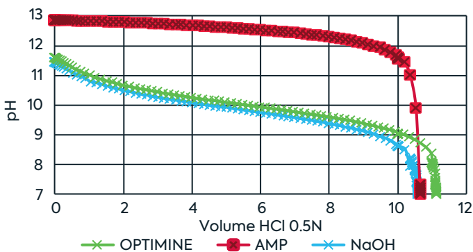
Fig. 5: Comparison of titration curves for OPTIMINE, AMP and NaOH.
