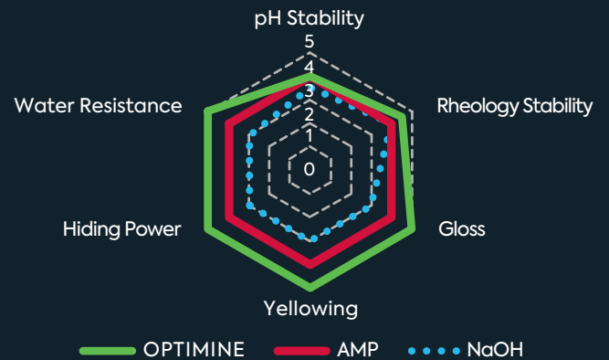
Fig. 1: Performance comparison of waterborne architectural paints formulated with OPTIMINE, AMP and NaOH.
